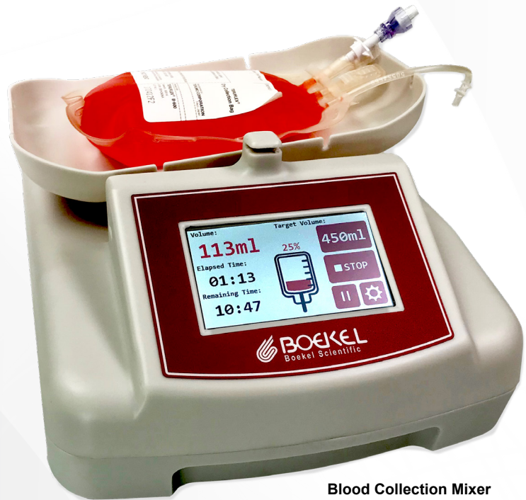
Blood Collection Mixer Part Number 30200
