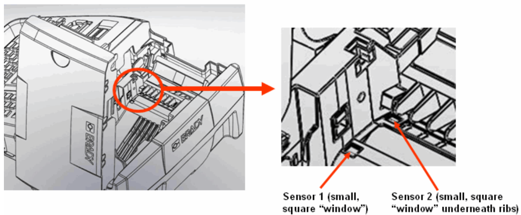
Figure 14 • Sensor locations
