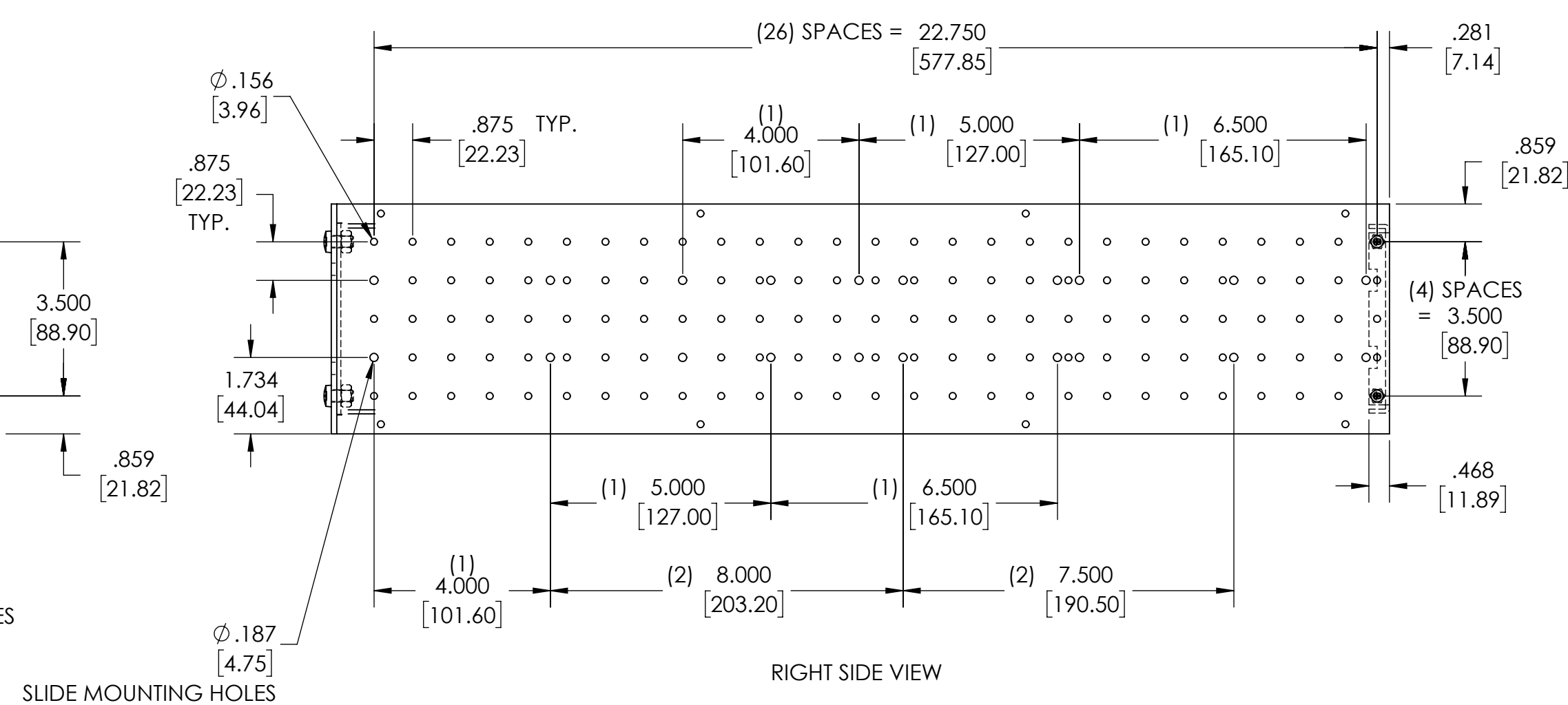
SLIDE MOUNTING HOLES
