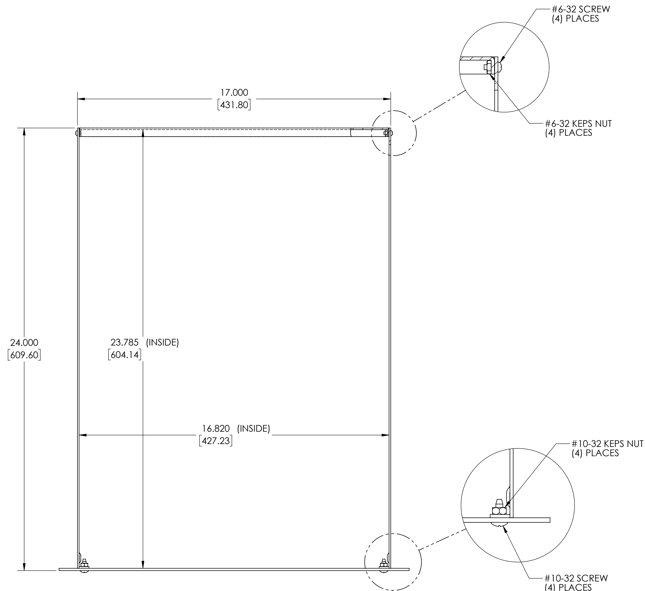
TOP VIEW
