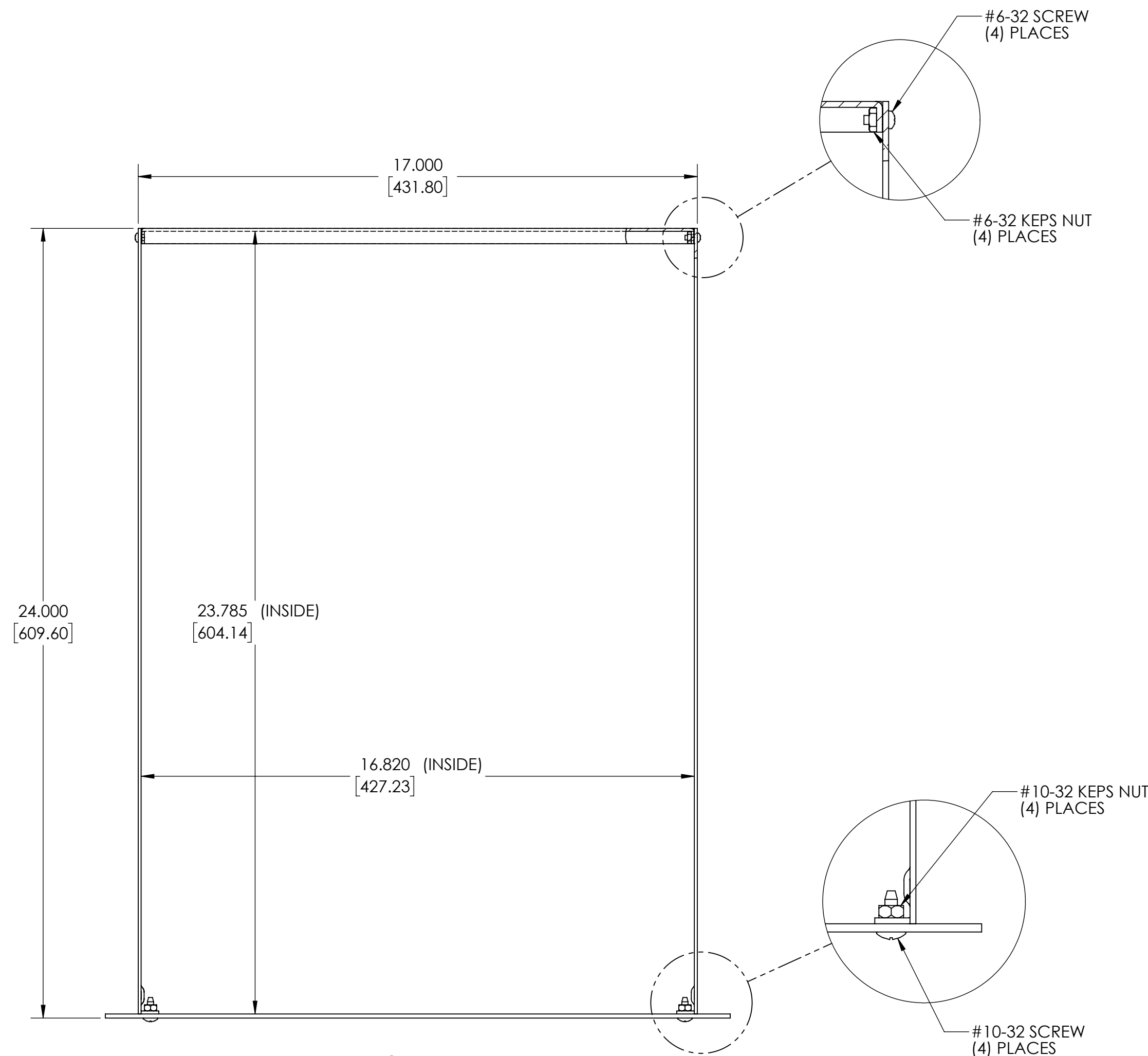
TOP VIEW
