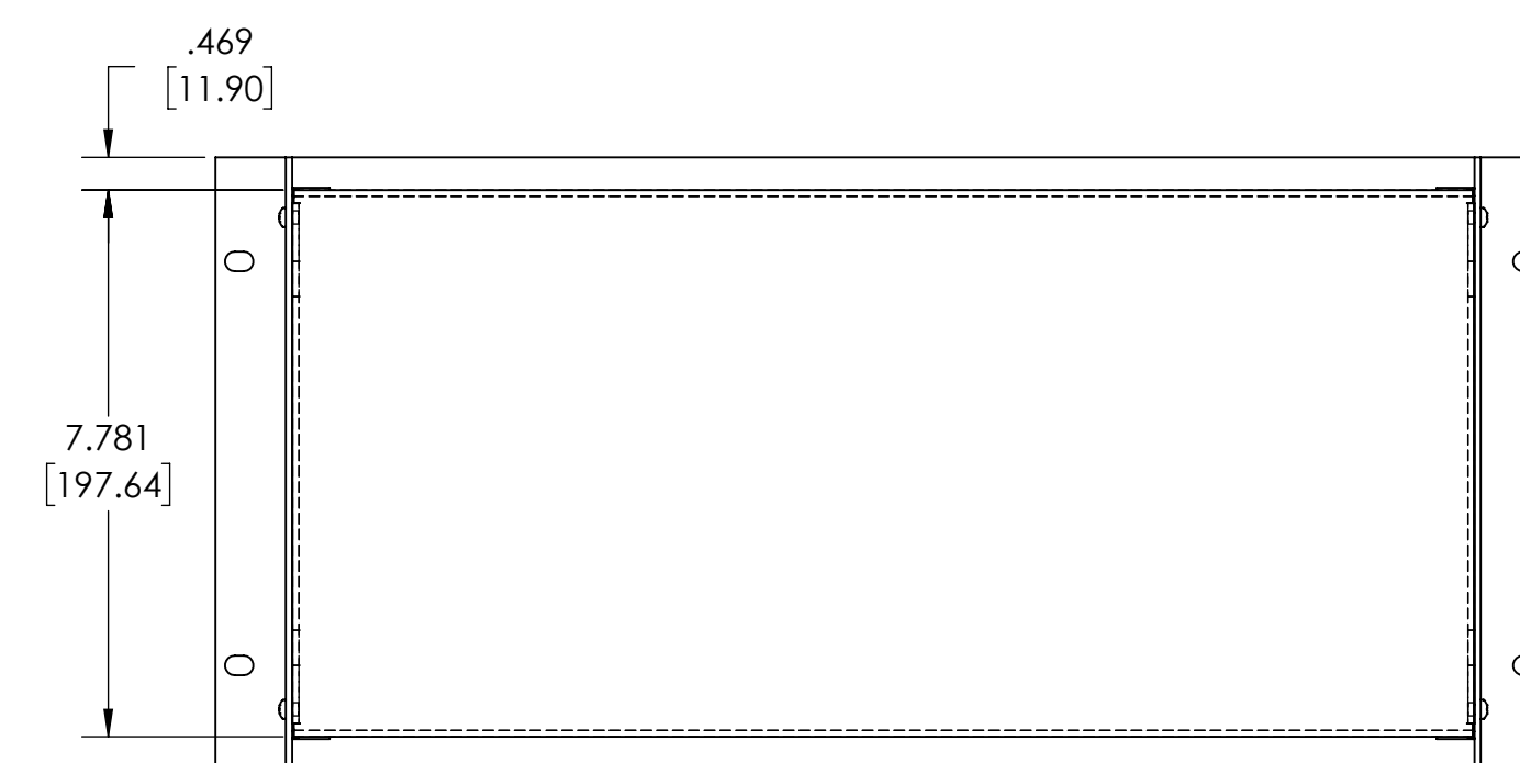
BACK VIEW
