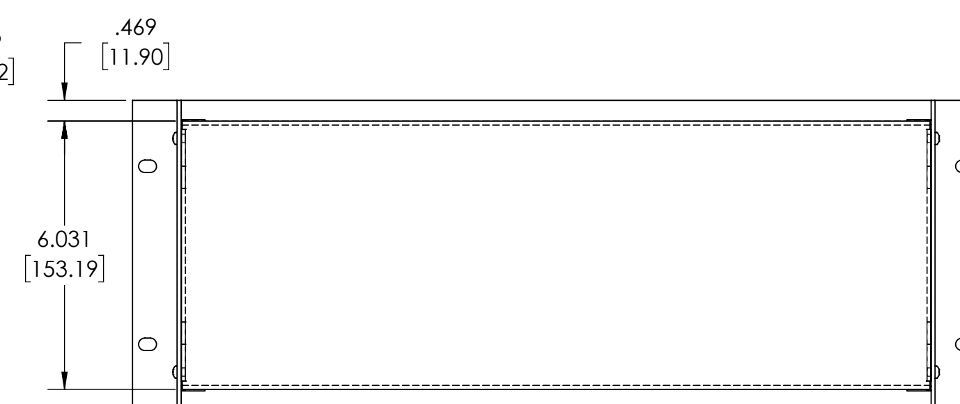
BACK VIEW
