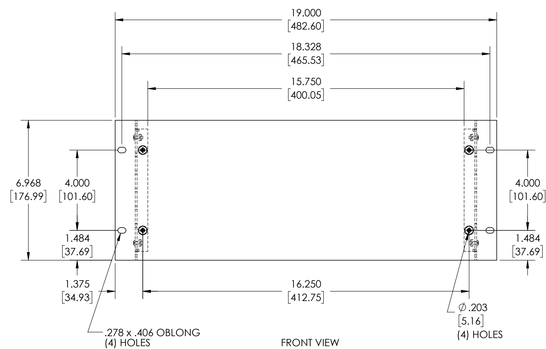
FRONT VIEW
