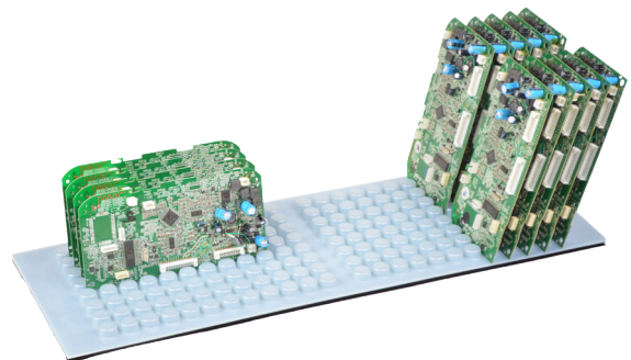
Dissipative IPA washable grid and CFP bottom.
