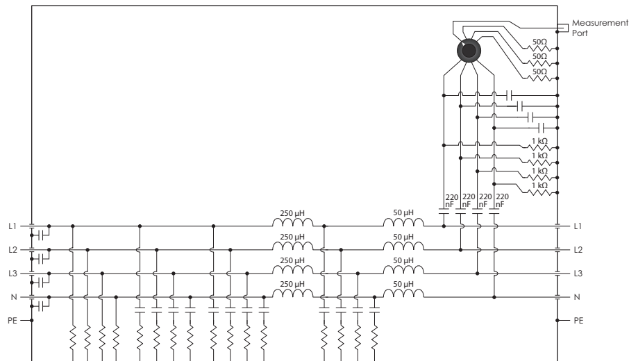
FIGURE 4 - Example Schematic of LI-3P-2x Series LISN
