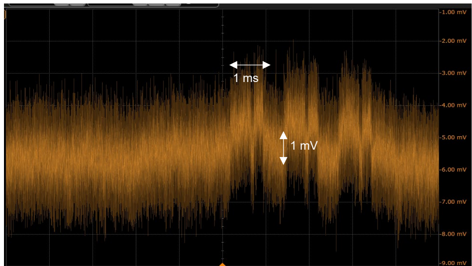
Figure 4. CX3300 captures very small differential voltage beyond a conventional differential probe
