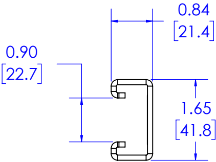
PROFILE VIEW 1:2
