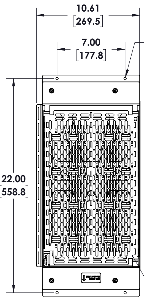
FRONT VIEW SLIDE CLOSED
