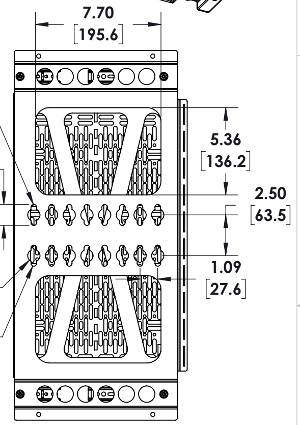
BACK VIEW SLIDE CLOSED
