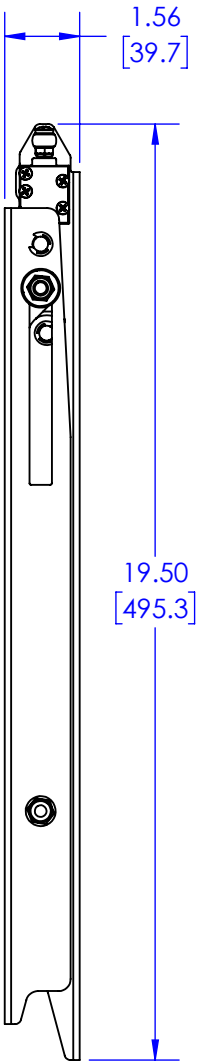
PLUMB AT 0°
