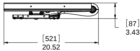
Retracted
