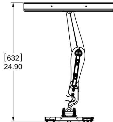
Extended
