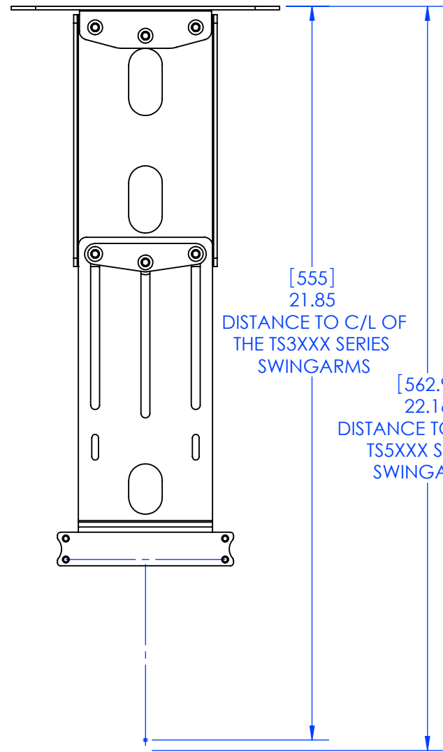
HIGHEST EXTENSION
