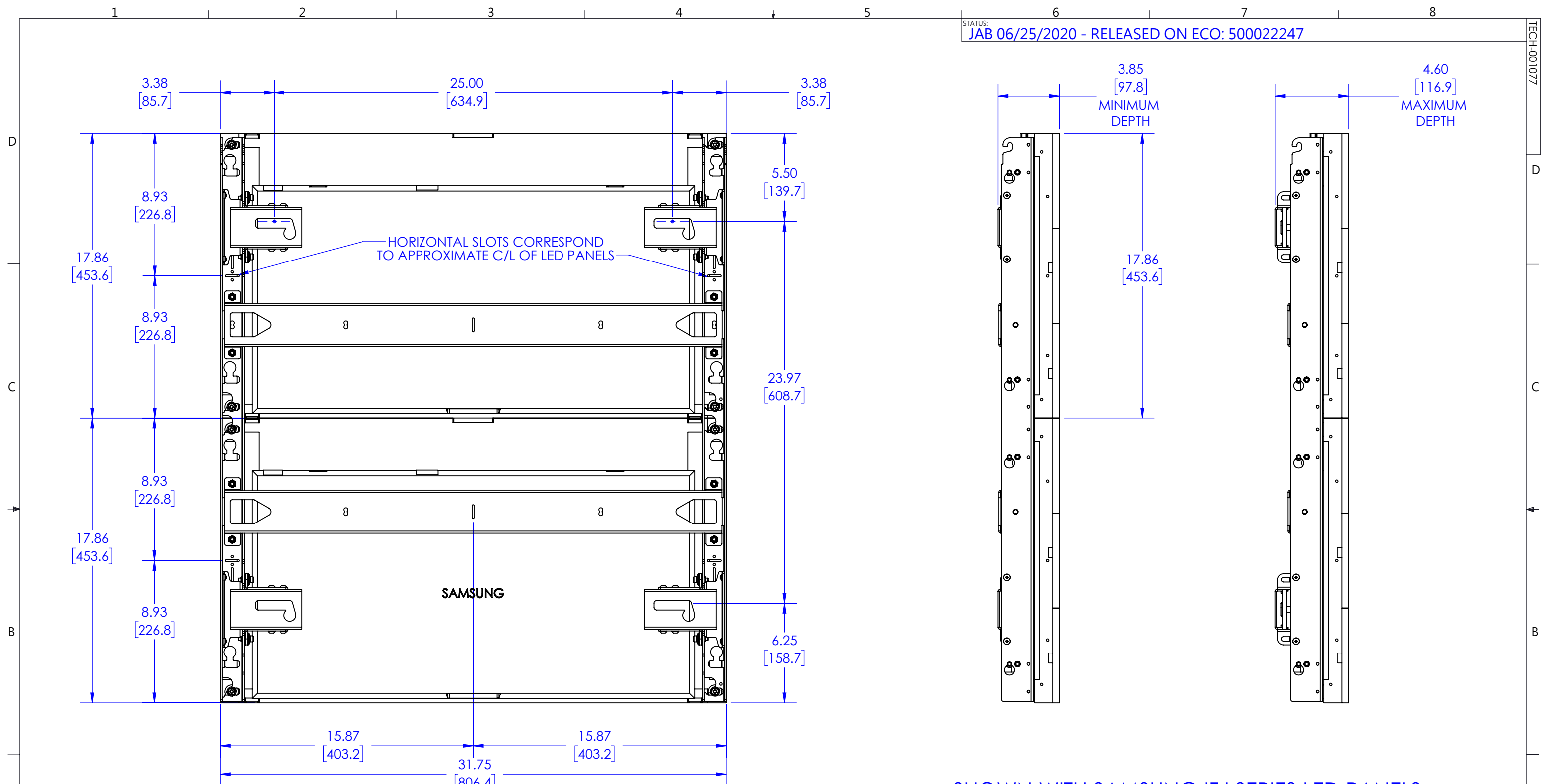
SHOWN WITH SAMSUNG IFJ SERIES LED PANELS
