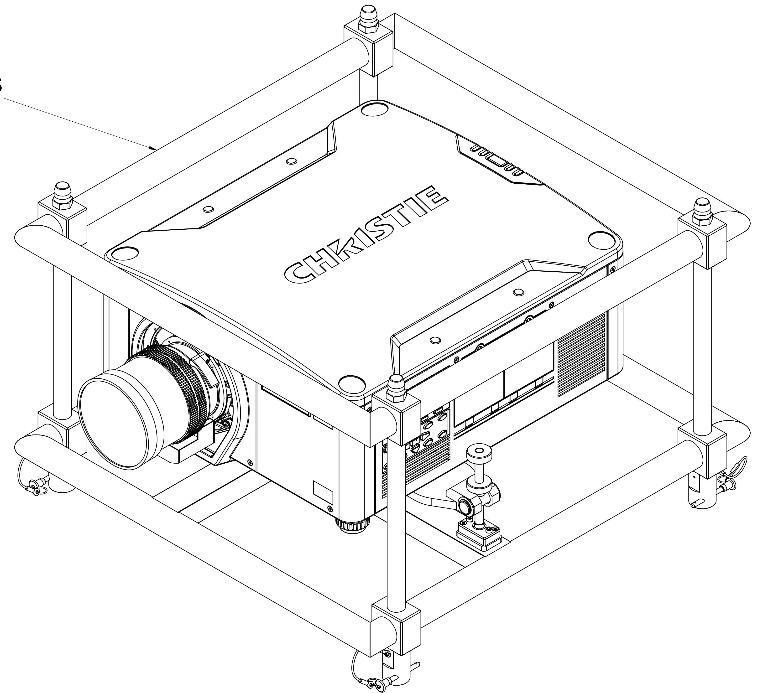
ISOMETRIC VIEW
