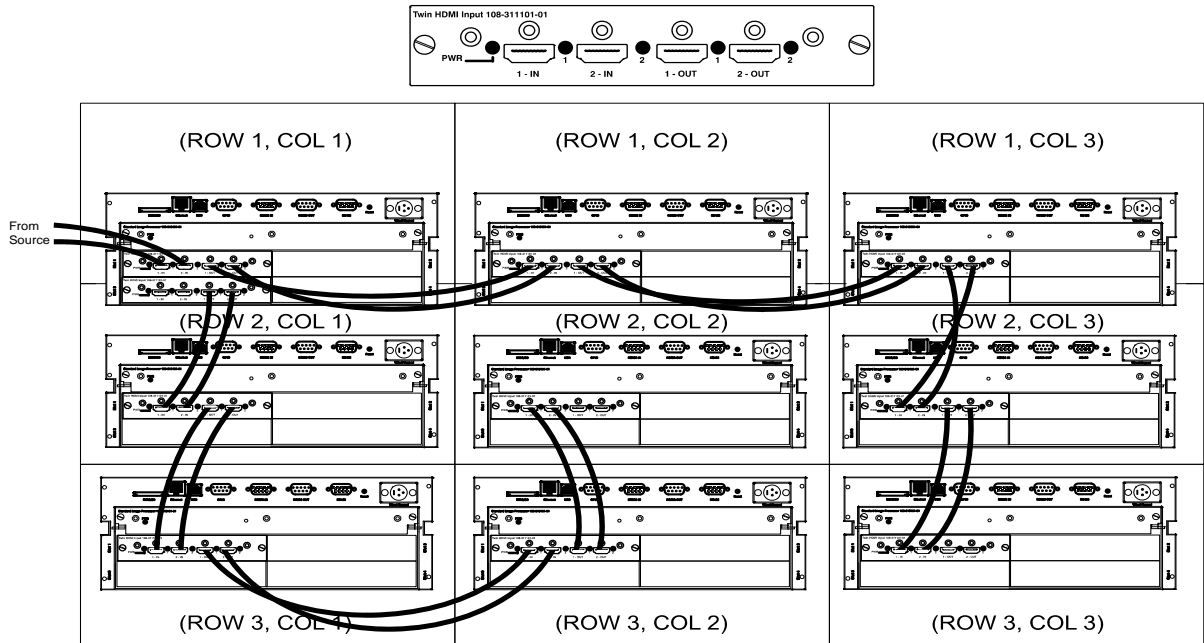
FIGURE 2-12 3X3 LOOP-THROUGH WIRING SOLUTION
