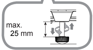
Front foot
