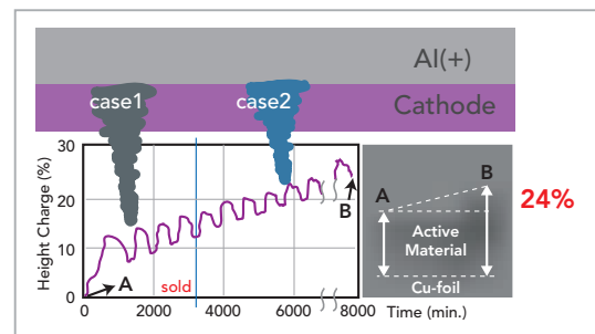
[Figure 5] Two burrs (case 1 & case 2) with different height extruded out from the aluminum positive electrode may cause internal short circuits in different time.
