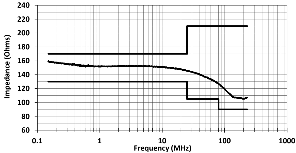
Figure 3 - Impedance compared to CISPR 16-1-2 edition 1.2 & IEC 61000-4-6 requirements.
