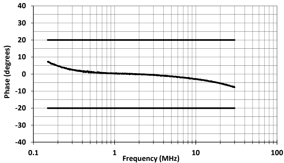
Figure 3 - Impedance compared to CISPR 16-1-2 edition 1.2 & IEC 61000-4-6 requirements.
