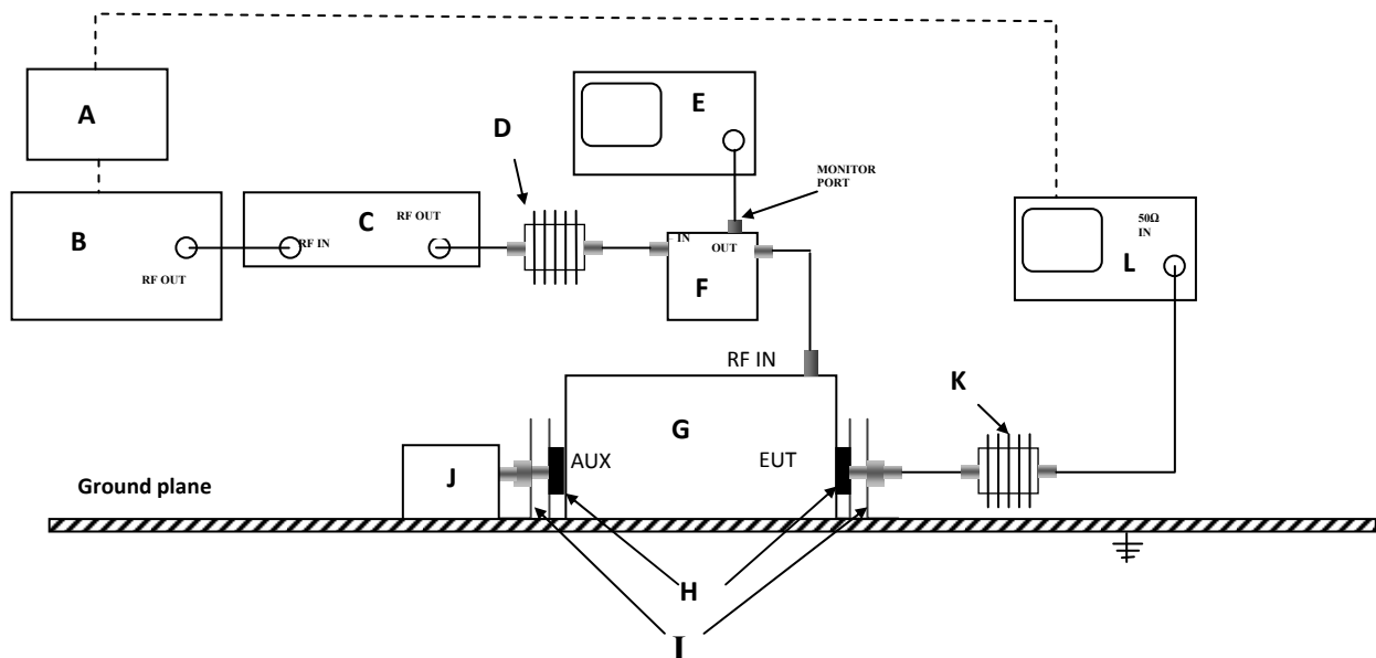
Figure 1: Typical Test level calibration setup
