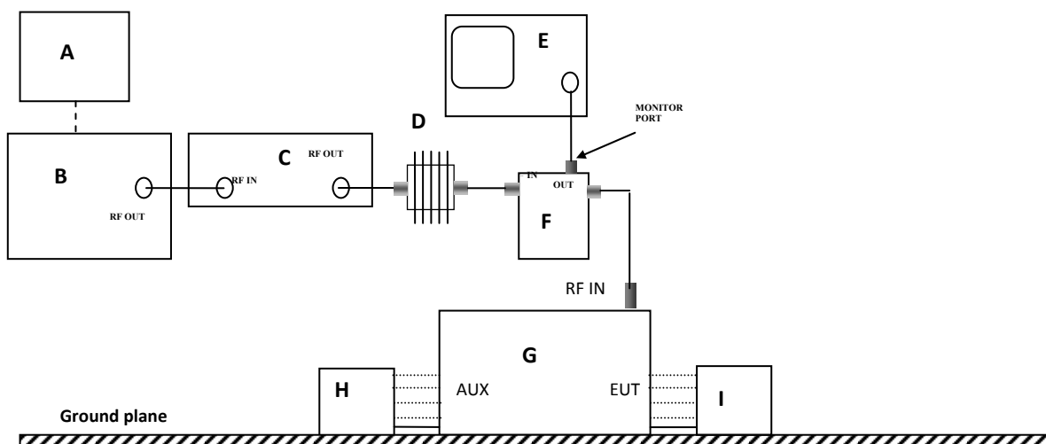
Figure 2: Typical Test Setup
