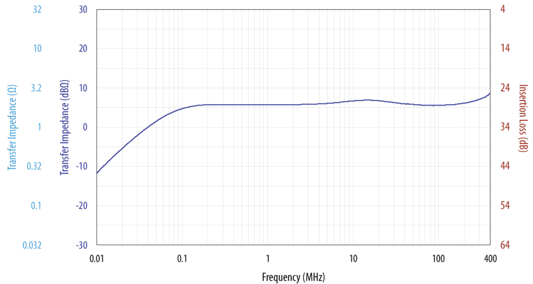
Figure 5 – Typical Insertion Loss/Transfer Impedance Factors for CLCE-452 Probe
