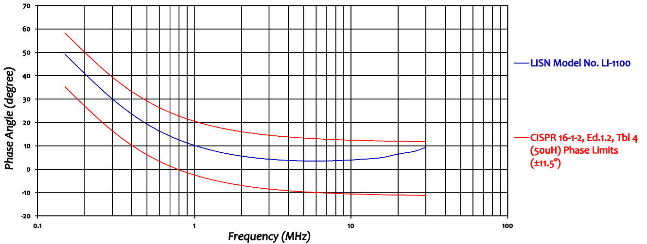
Figure 3 - Phase compared to CISPR 16-1-2 requirements.
