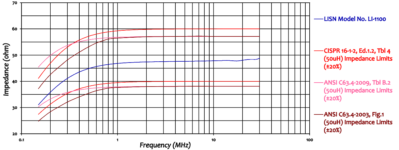
Figure 2 – Impedance compared to CISPR 16-1-2 and ANSI C63.4 requirements.
