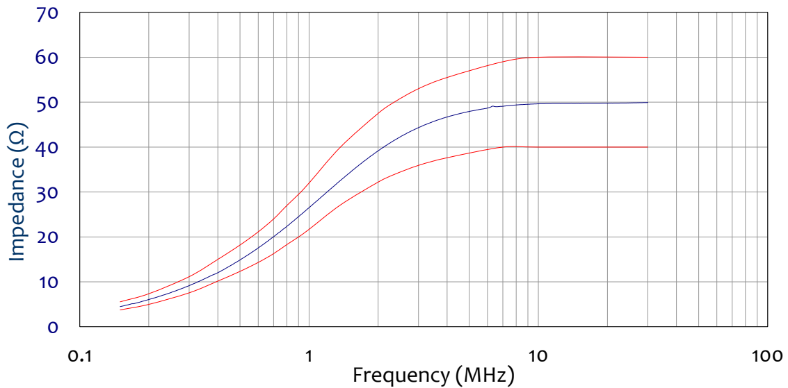
Figure 3 – Impedance (AE Port Open) compared to Mil-Std 461 requirements.
