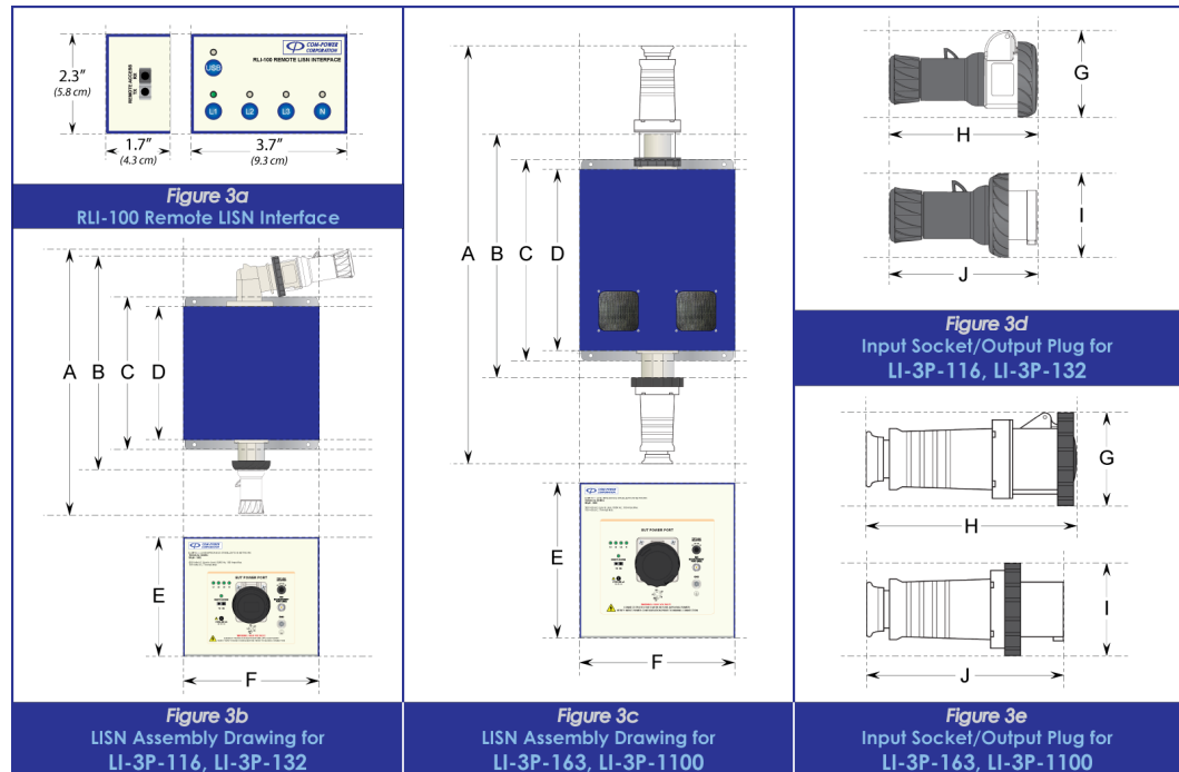
FIGURE 3 - Product Dimensions
