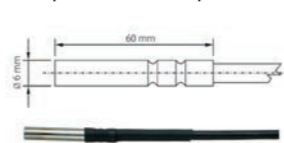
Pt1000TG68/E (-80°C to +200°C)
