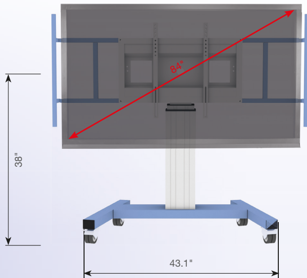
Lowest position – distance from floor to center of screen
