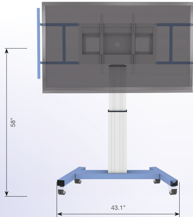
Upper position – distance from floor to center of screen
