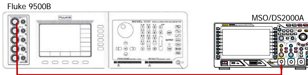
Figure 2-1 Impedance Test Connection Diagram
