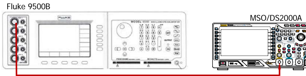
Figure 2-3 Bandwidth Test Connection Diagram
