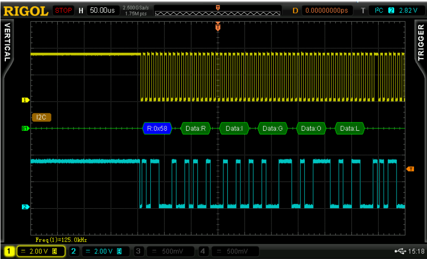
Figure 3-44 I2C Trigger and Decoding
