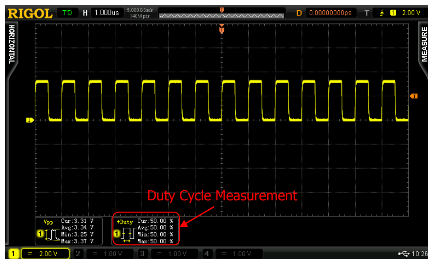
Figure 3-1 Demonstration Result of Square Waveform
