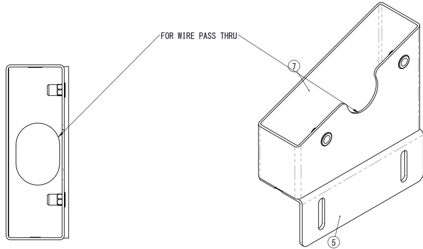
SLANT ADD-ON LEFT SIDE
