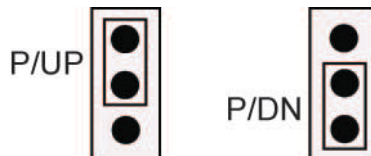
Figure 10. Pull-up/down jumper configuration
