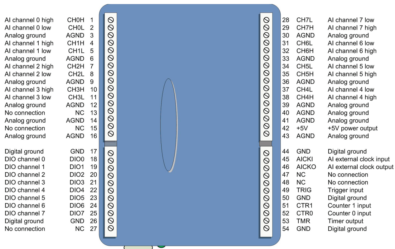
Figure 5. DIFF mode pinout
