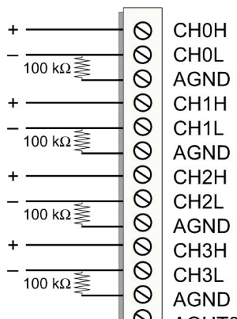
Figure 6. DIFF connections with ground path resistor
