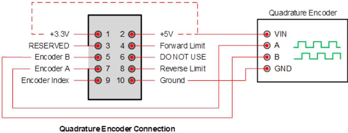
Figure 12.1 DMC60C Quadrature Encoder Connection
