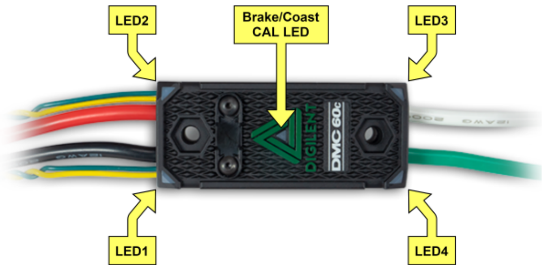
( https://reference.digilentinc.com/_media/dmc-60c/hardware-reference-manual/dmc60c-led-callout.png ) Figure 4.1 DMC60C LED Label Callout
