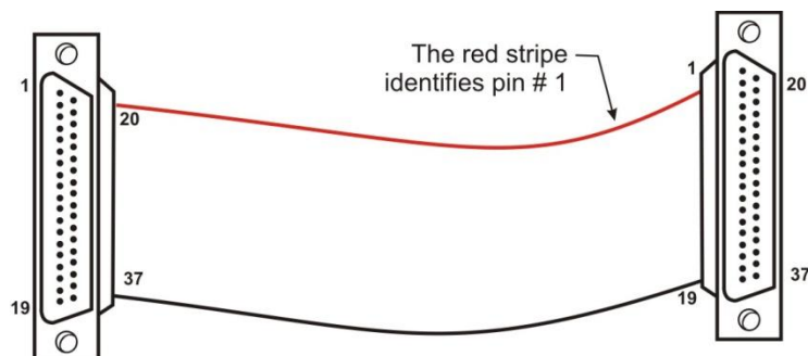
Figure 10. C37FF-x cable
