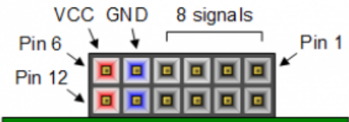
Figure 16. Pmod diagram.
