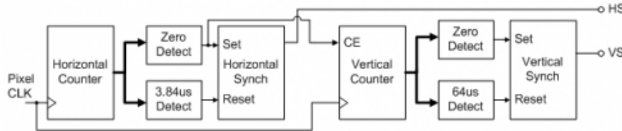
Figure 12. VGA display controller block diagram.
