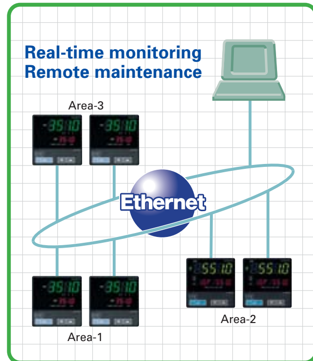
Direct Connection to Ethernet RJ45 connector-100Base-TX/ 10Base-T
