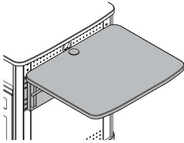
Flip-Up Shelf (mounts on left or right side, max two per unit) includes 2" grommet 23"W x 27 \frac{3}{8} "D (50 lbs max capacity) 55263
