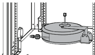
Retractable Cord Reel 15' retractable, 15-amp, 12 AWG, with breaker, UL listed 99029
