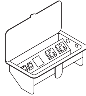
Power/Communication Module with 9' power cord, two outlets, and two data jacks 7 1/8"W x 3 5/8"D (standard models only) 99003 (without mic jack)
