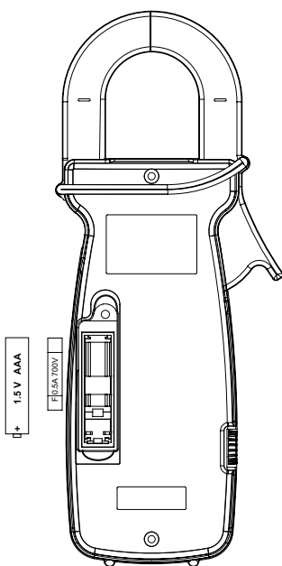
Fig. 4 Battery Fuse
