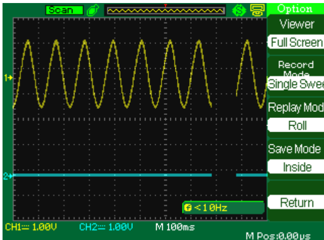
Figure 85 - Option Screen
