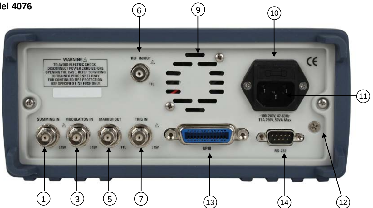
Figure 3.3 - Back Panel View
