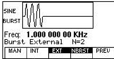
Trigger Menu
