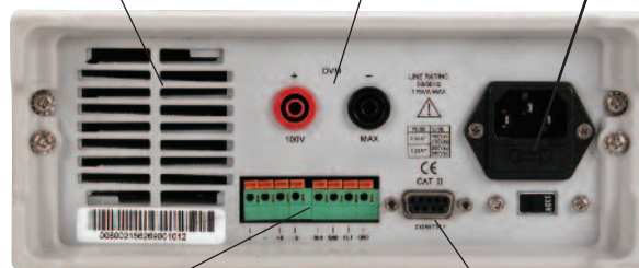
Remote Sense and digital port functionality
