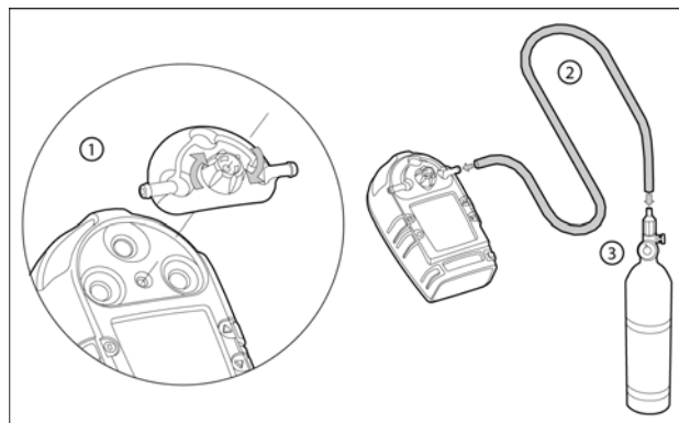
Figure 4. Attaching the Gas Cylinder to the Detector
