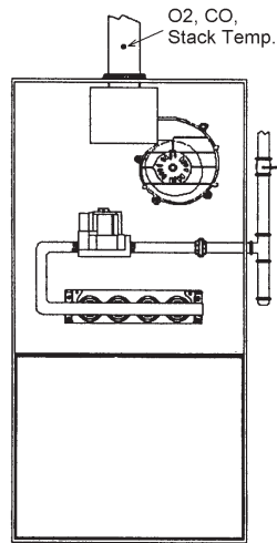
80% Eff. Fan Assist or Power Vented Furnace/Boiler
