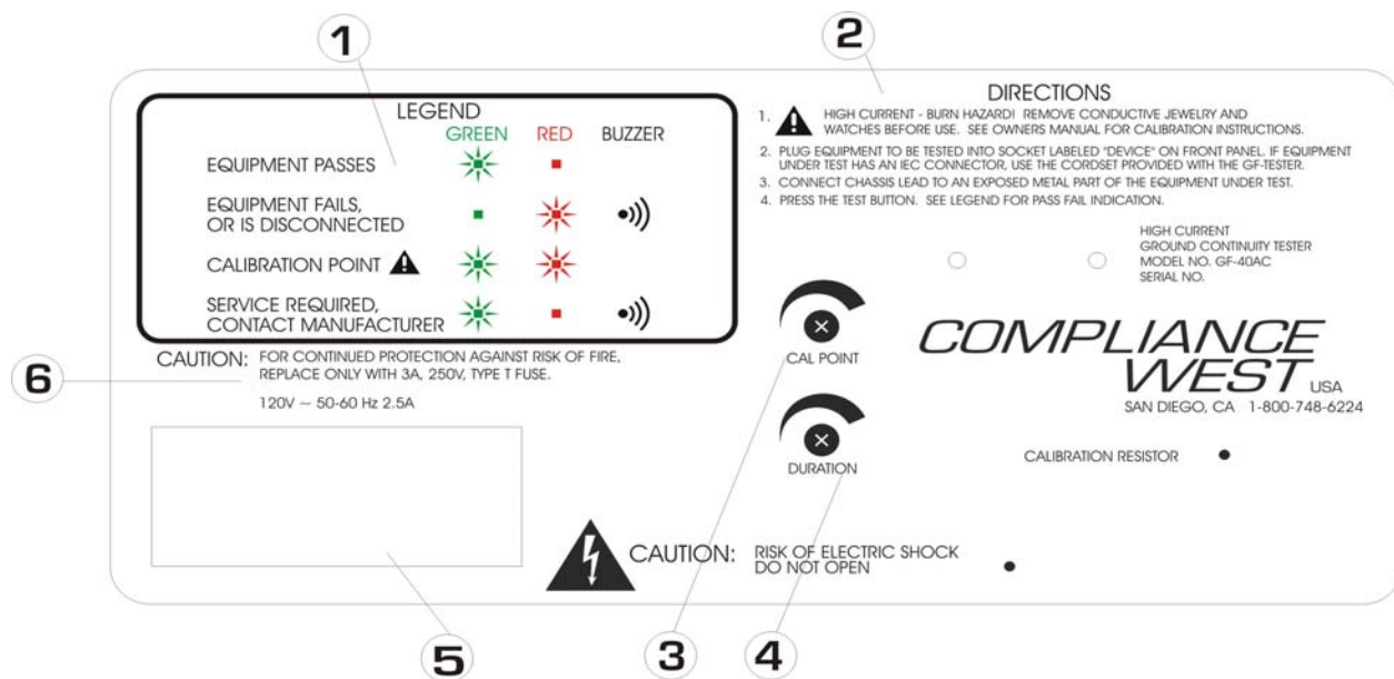
Figure 2-2. Control, Indicators, Connectors - Model GF-40AC Rear Panel
