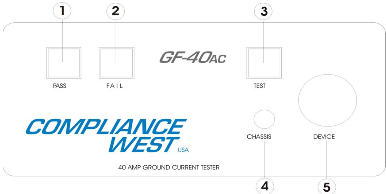
Figure 2-1. Controls, Indicators, Connectors - Model GF-40AC Front Panel
