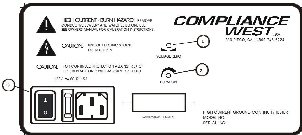
Figure 2-2. Controls, Indicators, Connectors - Model GFM-30ac Rear Panel
