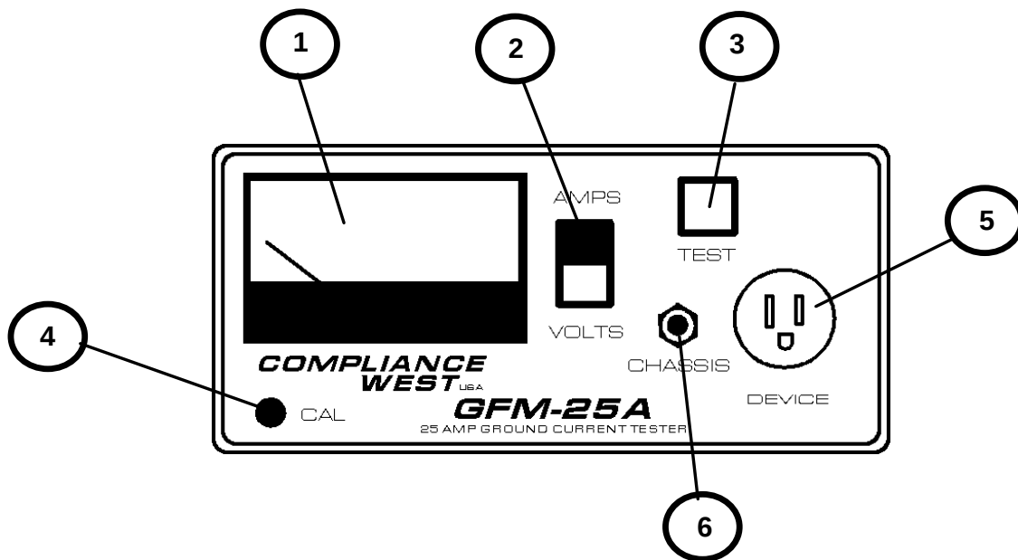
Figure 2-1. Controls, Indicators, Connectors – Example Model GFM-40ac Front Panel
