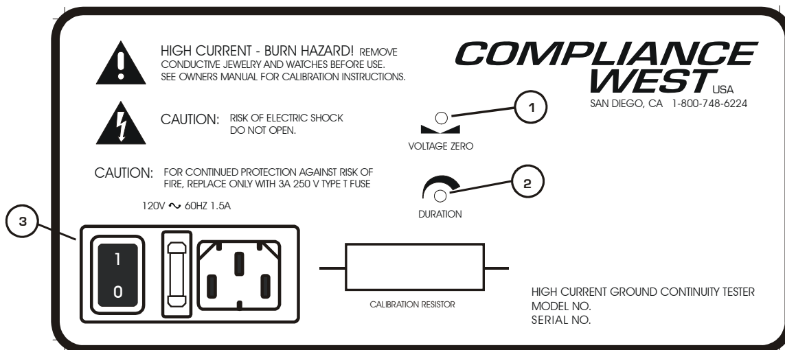
Figure 2-2. Controls, Indicators, Connectors - Model GFM-40ac Rear Panel
