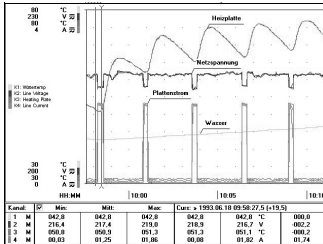
Y(t) Recorder Display for Up to 6 Channels
