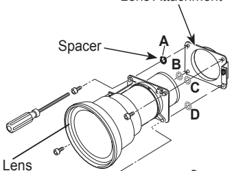
Lens Attachment
