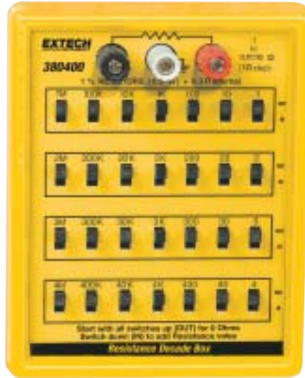
Model 380400 Resistance Box Features:
