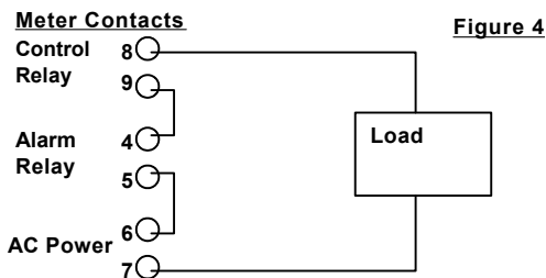
Figure 4 Wiring the Alarm and Control Relays in Series
